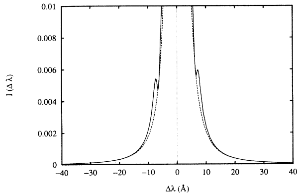
FIG. 2. Profile of the hydrogen L_\alpha line: ---, for thermal plasmas; —, for weakly nonthermal plasmas.
